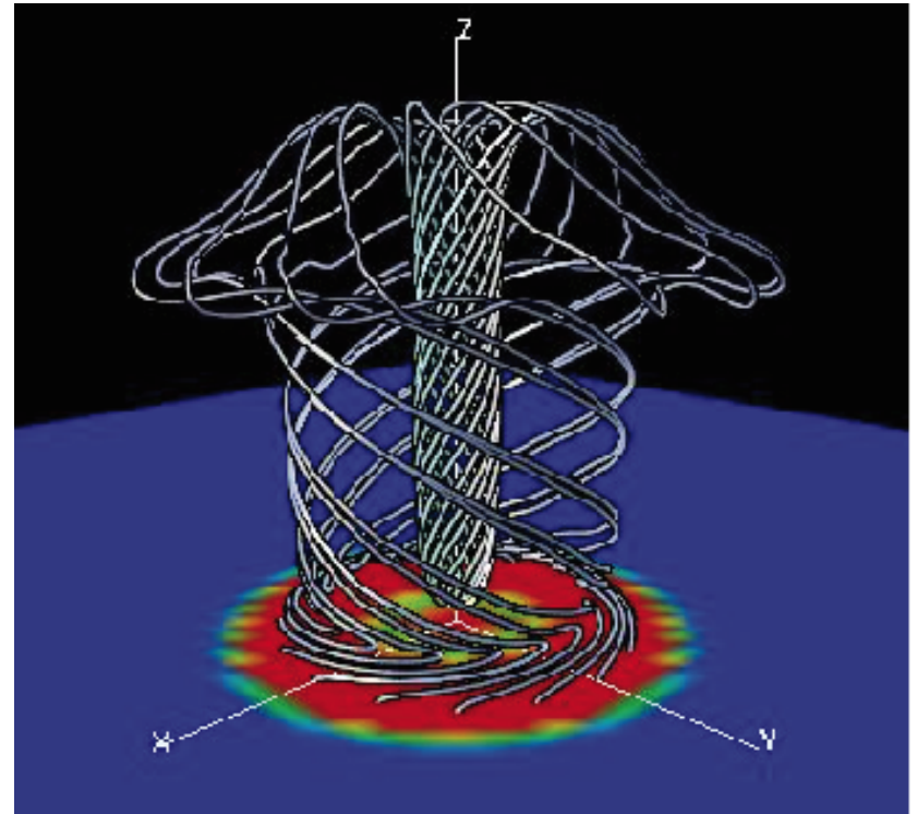
Magnetic tower jet
