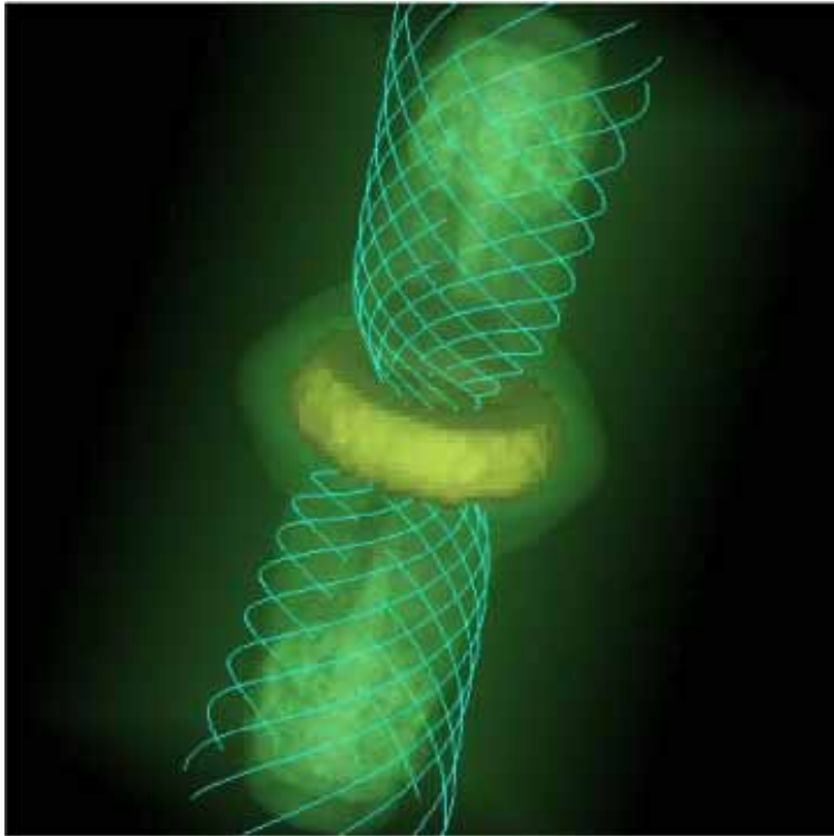
Magnetocentrifugal jet
